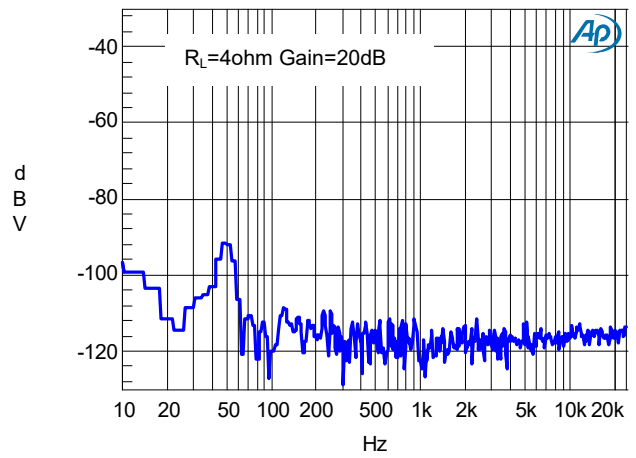
Noise Floor
